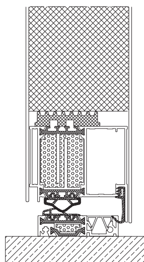
Aliplast GENESIS 75 mm
