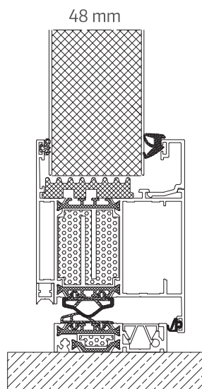
Aliplast GENESIS 75 mm
